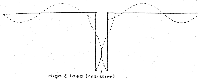
Fig. 6 — Current standing-wave distribution on the antenna and matching section at 21 MHz. On this band the antenna works as a long wire of five half waves. The base of the matching section presents a virtually nonreactive high impedance load to the feeder.
