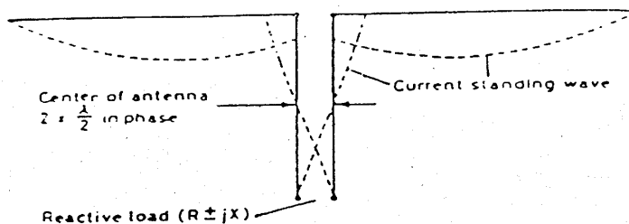
Fig. 2 — Current distribution on the antenna and matching section at 7 MHz. The antenna now functions as a collinear array with two half waves fed in phase.
