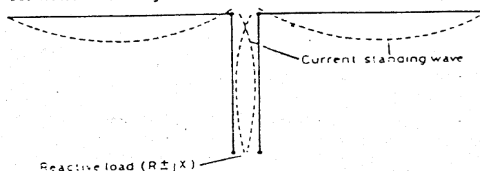
Fig. 3 — Current standing-wave distribution on the antenna and matching section at 10 MHz. The antenna functions as a collinear array with two half waves fed in phase.
