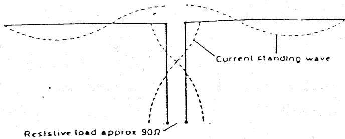
Fig. 4 — Current standing-wave distribution on the antenna and matching section at 14 MHz. In this case the antenna functions as a center-fed long wire of three half waves out of phase. The matching section now functions as a 1:1 impedance transformer, presenting a resistive load of approximately 90 ohms at the lower end.
