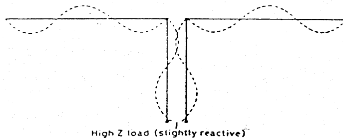
Fig. 8 — Current standing-wave distribution on the antenna and matching section at 28 MHz. The antenna functions as two long-wire antennas each of three half waves length, fed in phase. A very effective form of antenna giving good multilobe, low zenithal angle, radiation.
