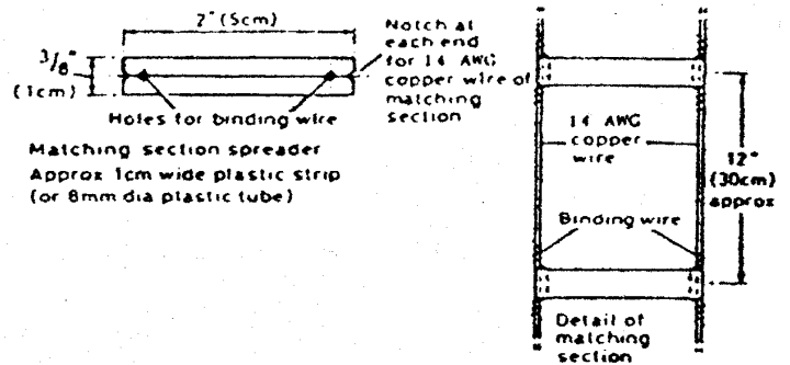
Fig. 10 — Constructional details of the matching section. Also suitable for open-wire feeder construction.
