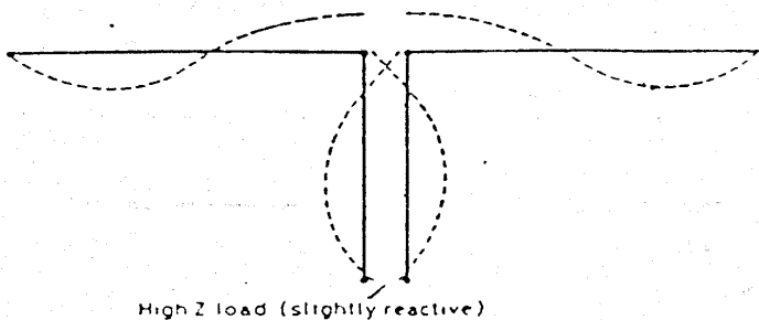
Fig. 5 — Current standing-wave distribution on the antenna and matching section at 18 MHz. The antenna functions as two full-wave antennas, slightly folded up at the center, fed in phase.
