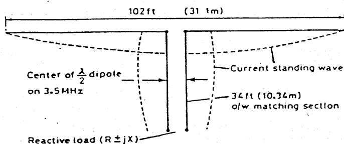
Fig. 1 — Current standing-wave distribution on the G5RV antenna and matching section at 3.5 MHz. The antenna functions as a \lambda/2 dipole partially folded up at the center.
