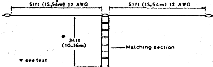
Fig. 9 — Construction dimensions of the G5RV antenna and matching section.
